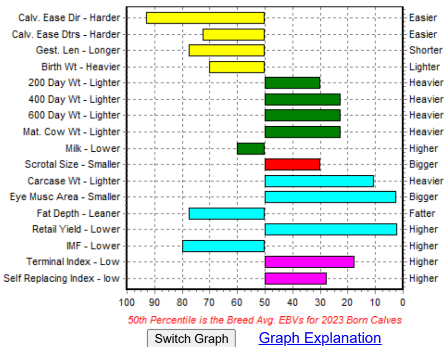
EBV Percentiles for RAWBURN EVOLUTION U837
